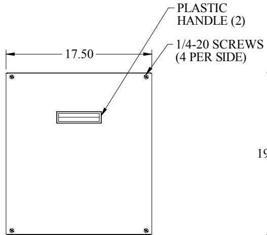
L.S. VIEW
